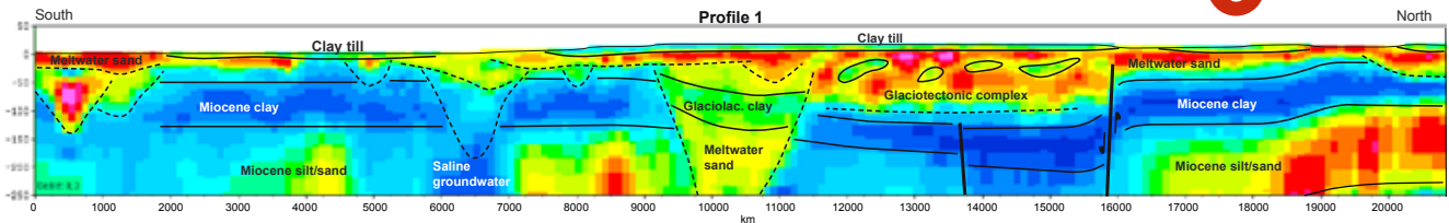
Source: Jørgensen et al. 2012: Transboundary geo-physical mapping of geological elements and salinity distribution critical for the assessment of future sea water intrusion in response to sea level rise. Hydrology and Earth System Sciences, 1845-1862.
